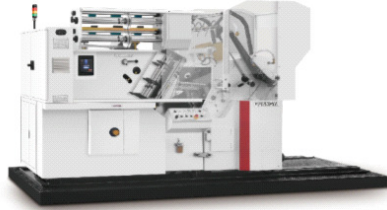
TL780 – Automatic Foil Stamping and Die Cutting Machine, format 78 x 56 cm, 3 reels
